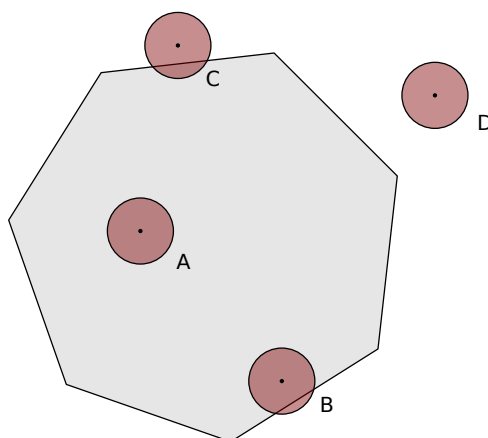
Figure 164: Example image used for circle/polygon collision detection
